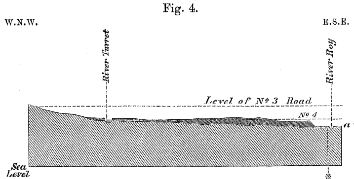
Section of Glen Turret detrital terrace mound from the Turret at the foot of the pass into Glen Gluoy to the River Roy, a distance of 1 mile.
