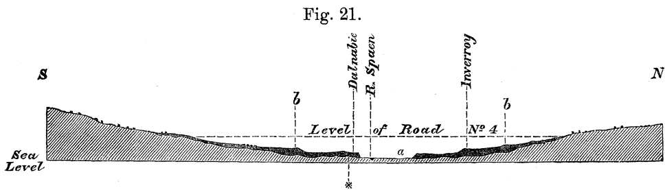
Section across the Spean at Inverroy near Roy Bridge. a. River gravel. b. Moraine detritus and gravel (represented somewhat too thick). * Ice-worn surface of rock.
